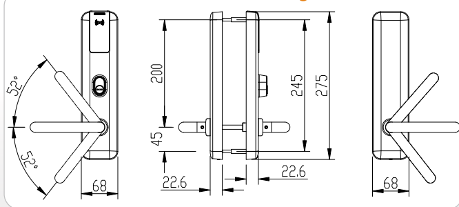
Technical Drawing
