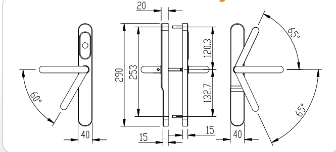
Technical Drawing
